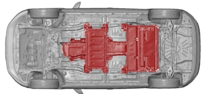
Battery pack
