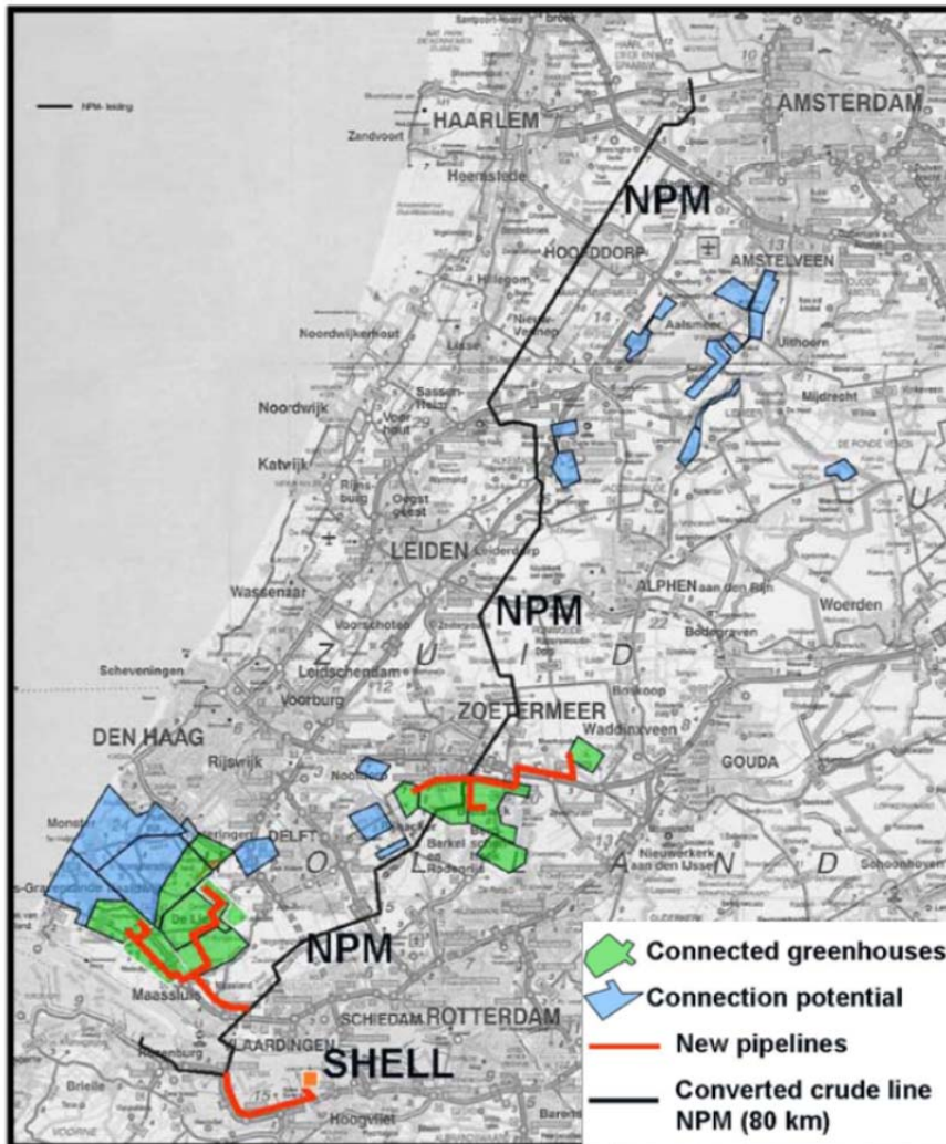
Figure 3.6: OCAP pipeline with connected greenhouse areas
