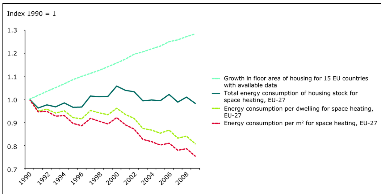
Figure 6.1. Trends in heating energy consumption and energy efficiency. (EEA, 2010)
